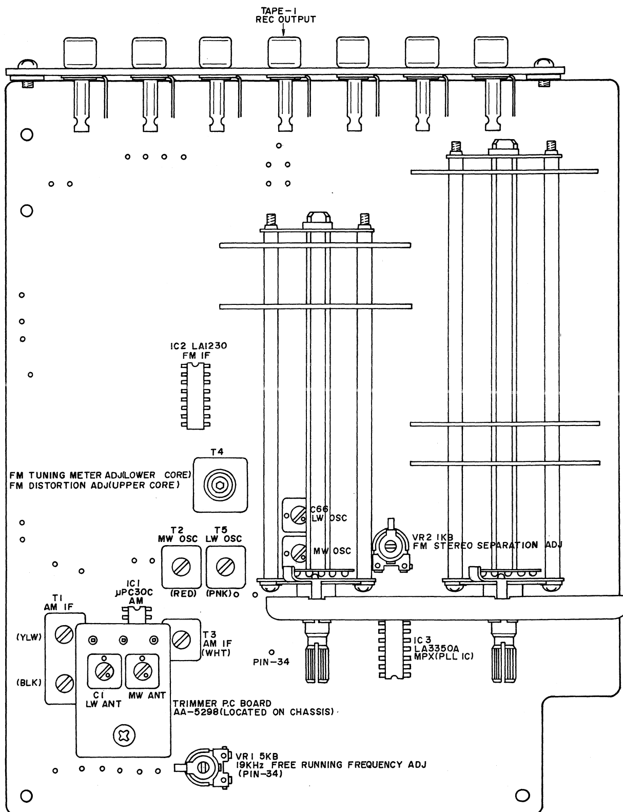
Fig. 2 MFC P.C Board AA-5270A (AA-1030L)
