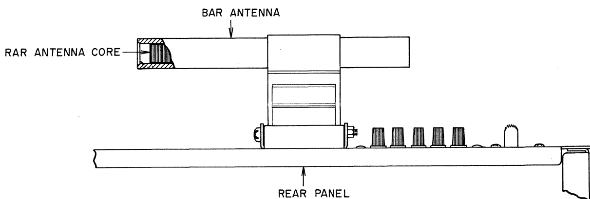
Fig. 5 Model AA-1030
