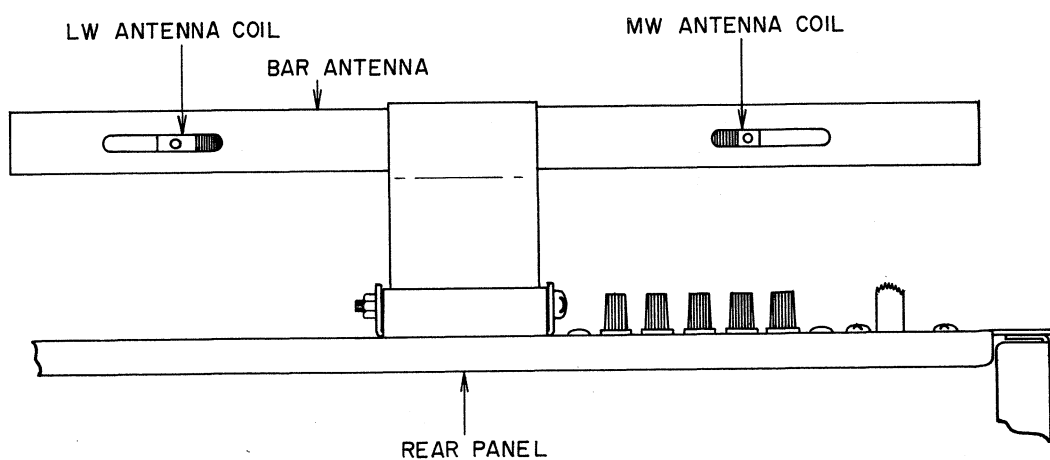
Fig. 6 Model AA-1030L
