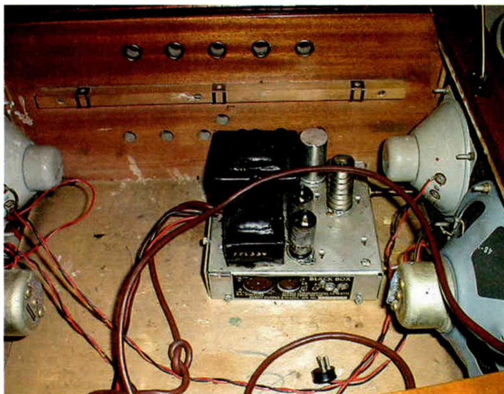
The amplifier refitted in the Black Box cabinet.
