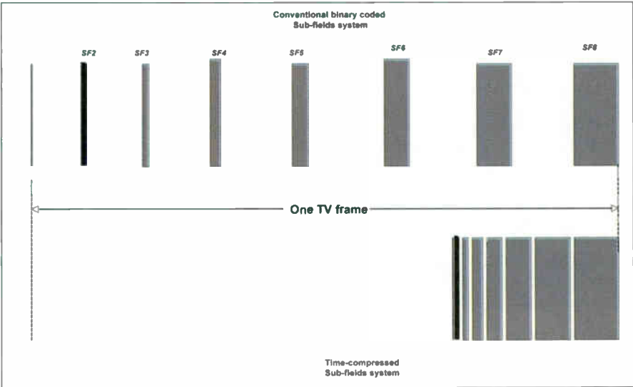
Fig. 3: Time-compressed sub-fields.
