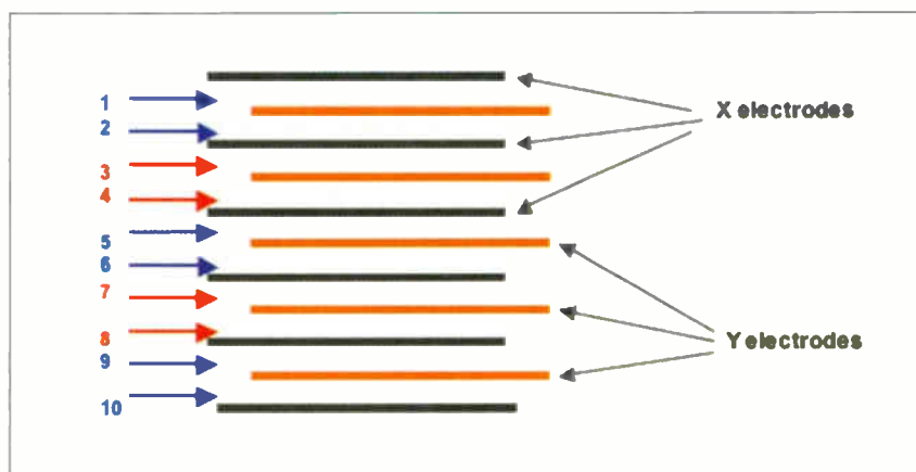
Fig. 11: Enhanced-ALIS drive.
